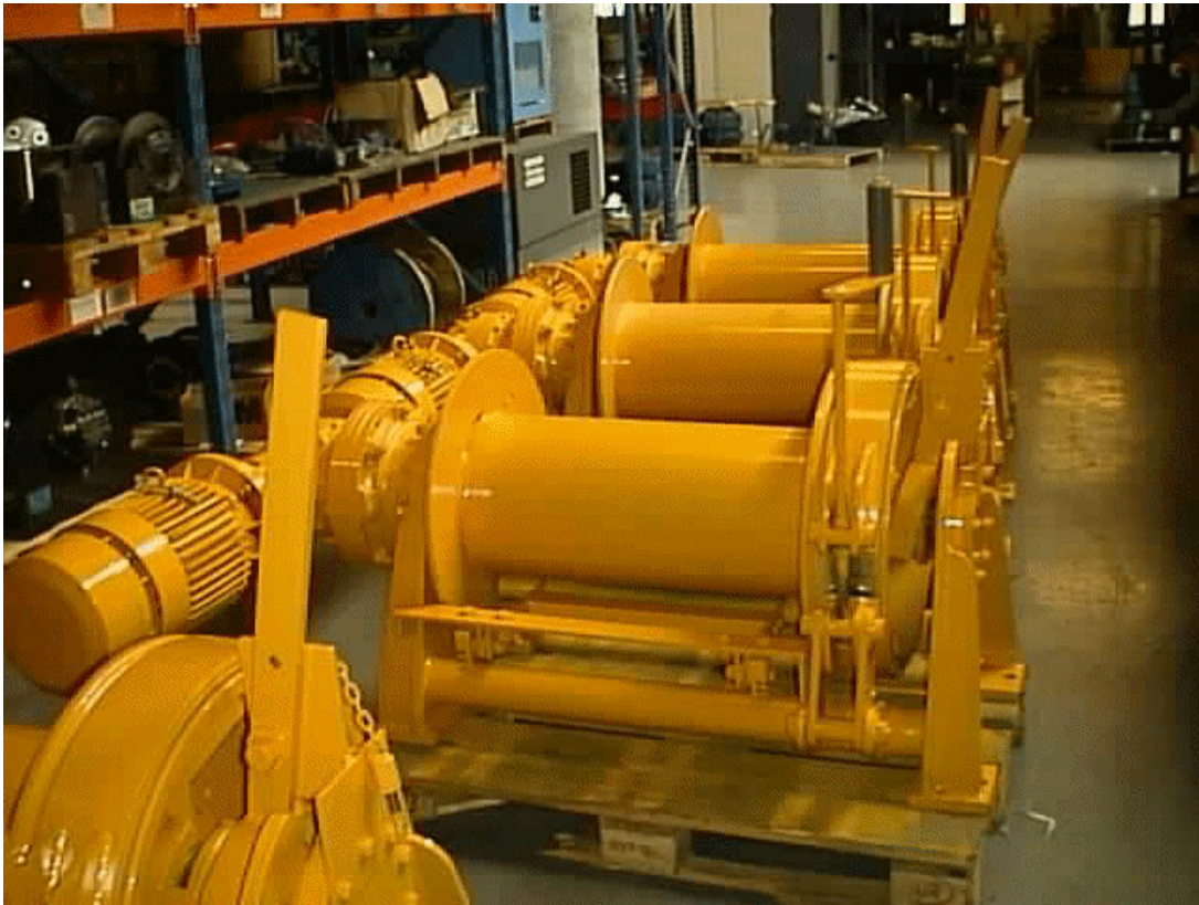
Electric planetary mooring winch
